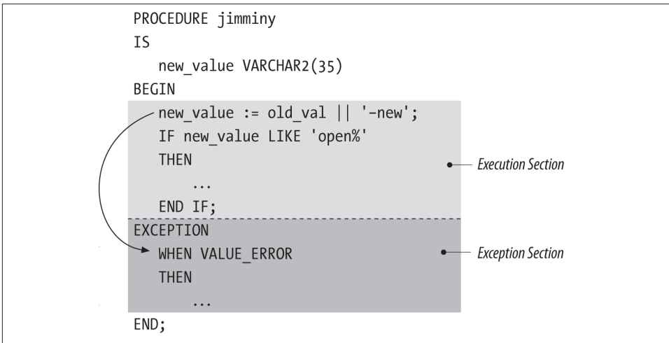
Figure 6-1. Exception-handling architecture
